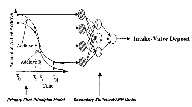
Figure 3. Hybrid neural network for IVD prediction.
