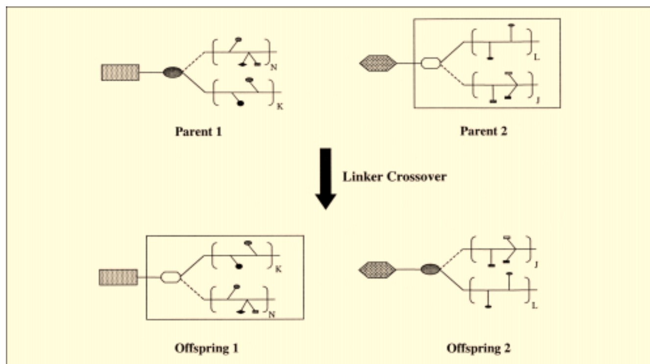
Figure 21. Linker crossover operator.
