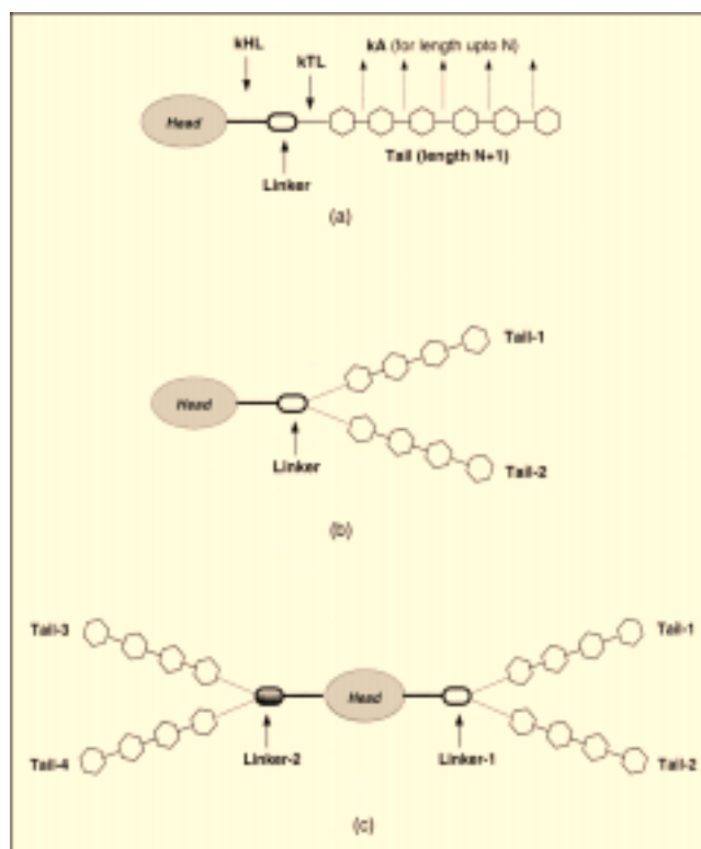
Figure 4. Generic structure of fuel additives.
