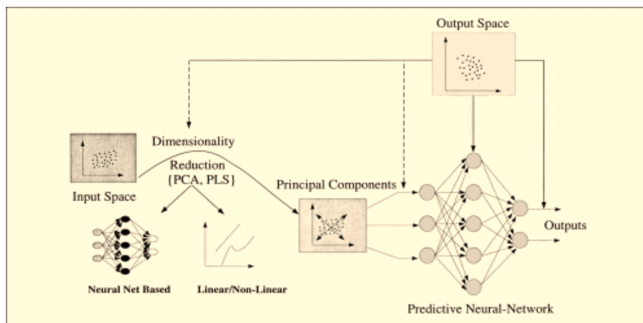
Figure 11. General architecture of neural networks considered in the BMW database.
