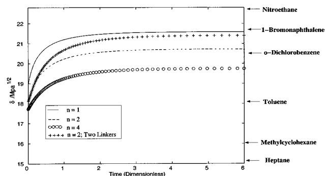
Figure 8. Solubility parameter vs. time for additives with different structures.
