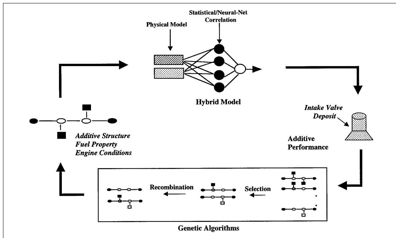
Figure 16. Forward and inverse problems in computer-aided fuel-additive design.
