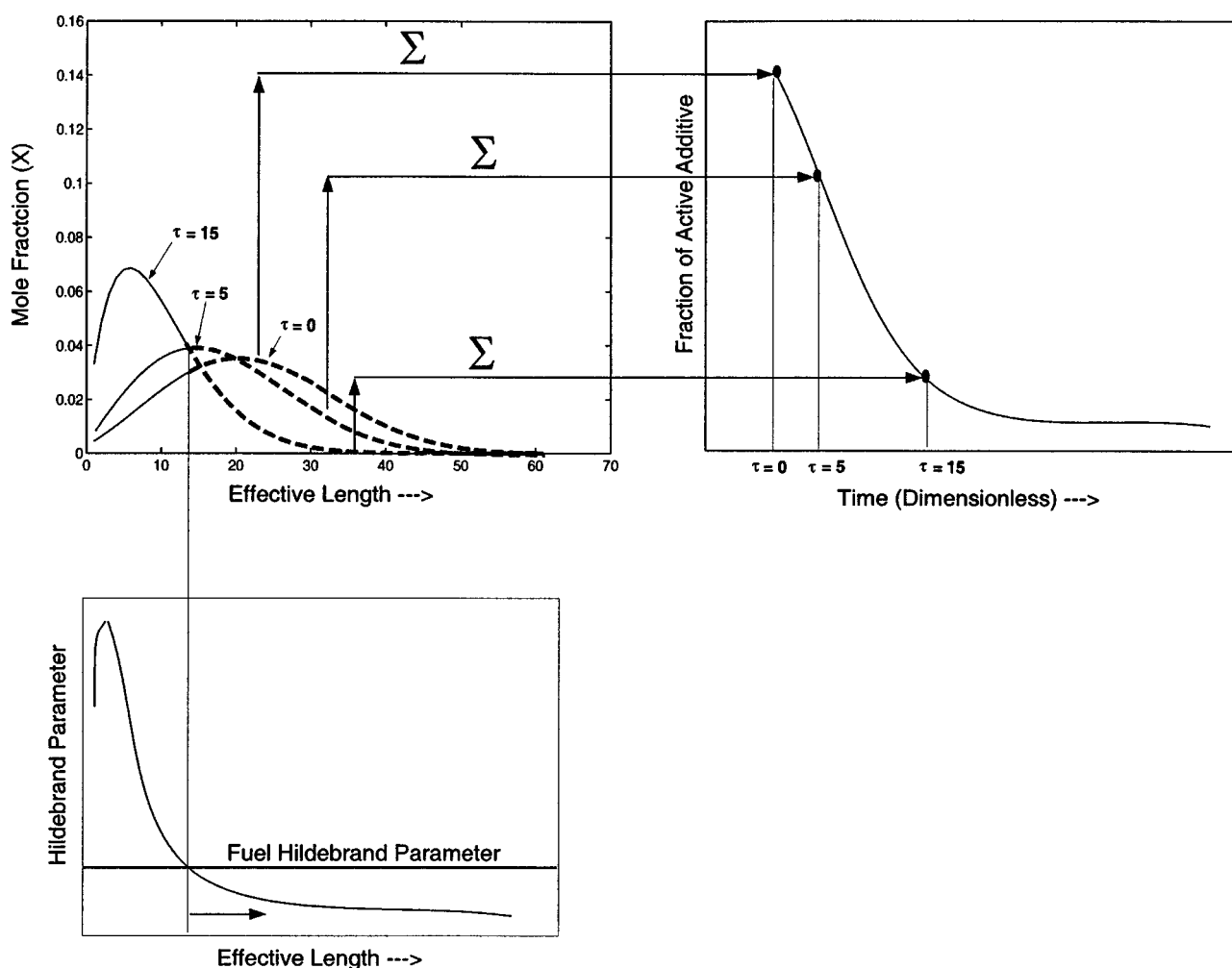
Figure 10. Determination of amount of active additive from solubility distribution.
