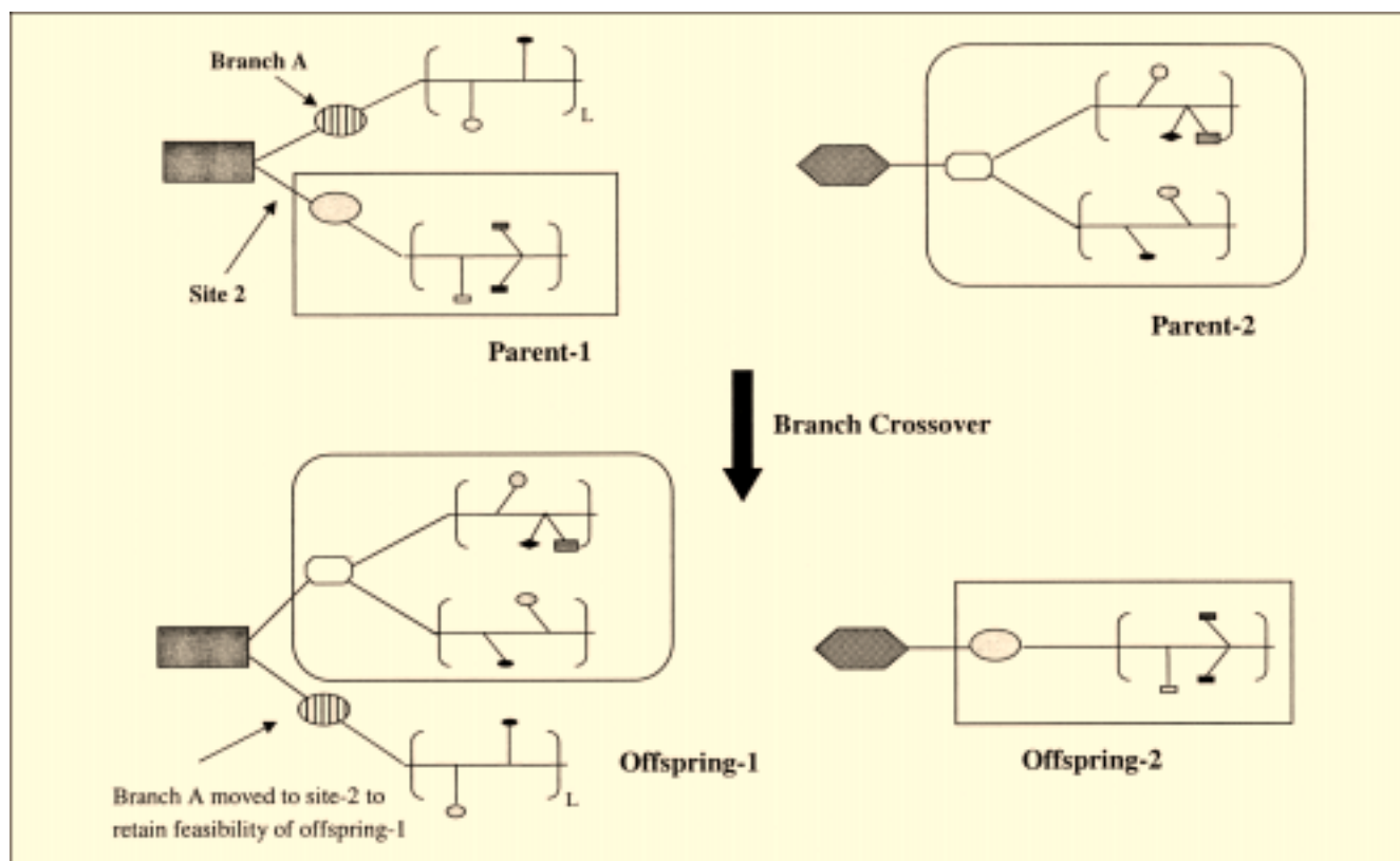
Figure 20. Branch crossover operator.
