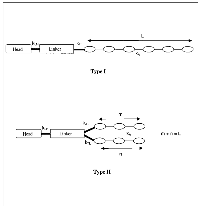
Figure 5. Type I and Type II structures.
