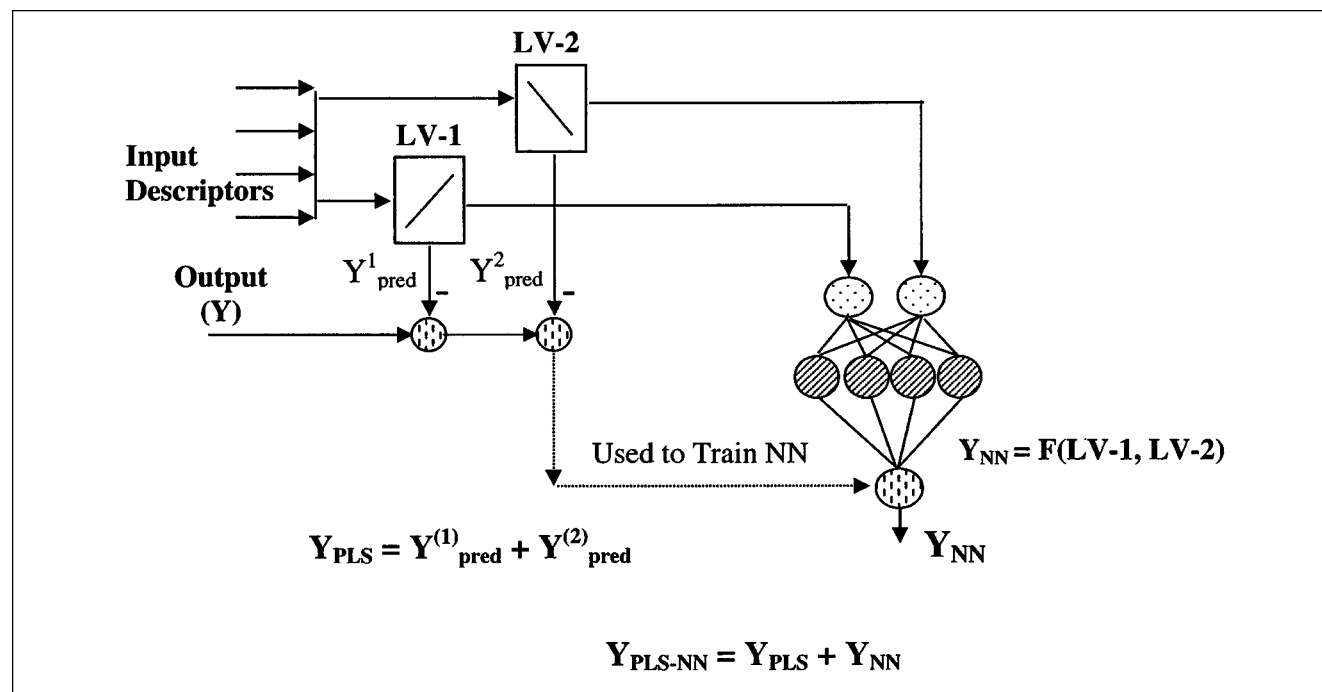
Figure 13. General architecture of a PLS-NN model.
