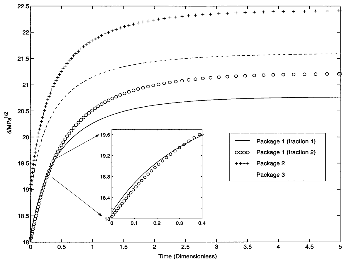
Figure 9. Solubility parameter variation with time for different additives (BMW database).
