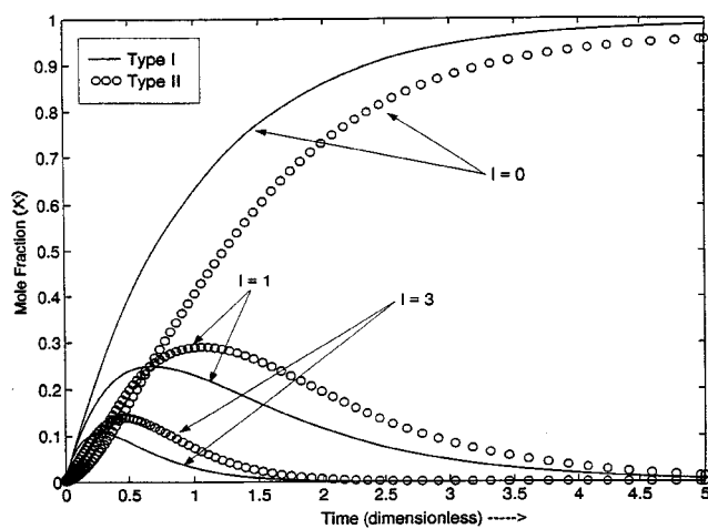
Figure 6. Comparison of degradation behavior of different chain-length additives.
